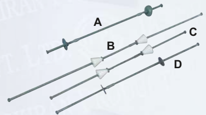
MODEL: JPPL-1506A,B,C,D SNAP TIES WITH PLASTIC CONES & WITHOUT PLASTIC CONES
