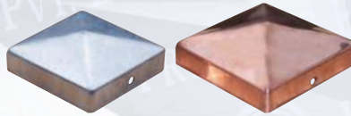
MODEL: JPPL-1407 POLE-POST CAP PYRAMID TYPE AVAILABLE IN COPPER, ALUMINIUM, COLORED POWDER COATED & HOT DIP GALVANISED. POST SIZE: 71x 71mm, 77x 77mm, 91x 91mm, 97x 97mm, 101x 101mm, 104x 104mm, 141.5 x 141.5mm
