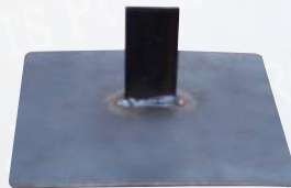
MODEL: JPPL-1201 BASE PLATE 150x150x2mm With STRIP
