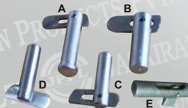
MODEL: JPPL-1614 A,B,C,D,E BRACE LOCKS ROD Ø 12mm, 16mm, 20mm.
