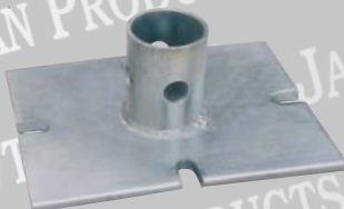
MODEL: JPPL-1206 SHOREX PLATE WITH PIPE SIZE: 9" x 6 3/4" x 3/8"
