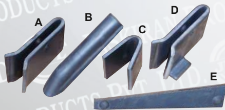
MODEL: JPPL-1751A,B,C,D,E QUICK STAGE ACCESSORIES A) "U" CLIP B) GUIDE PIN , C) "V" CLIP, D) TRANSUM , E) TAPER WEDGE 6 mm.
